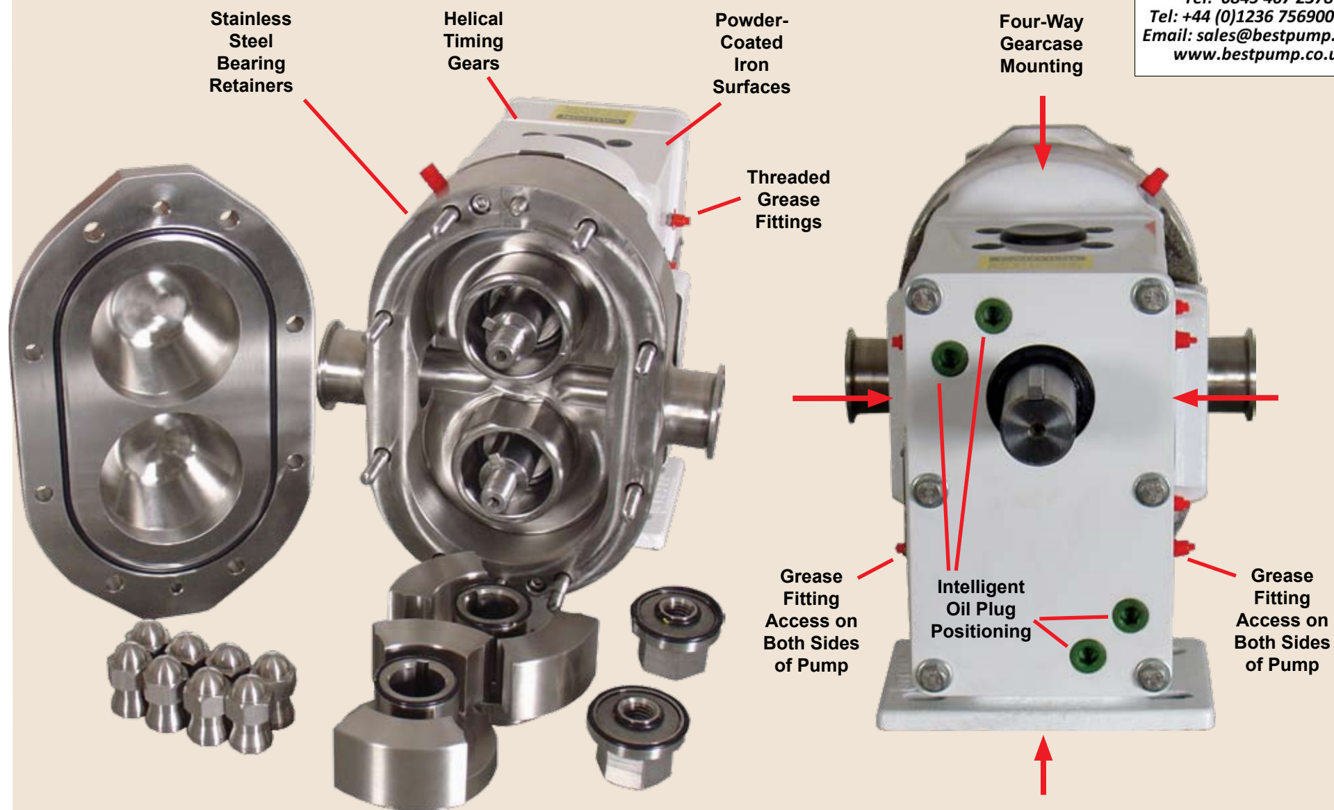
WRIGHT TRA20 Series (Clean in Place Option)
